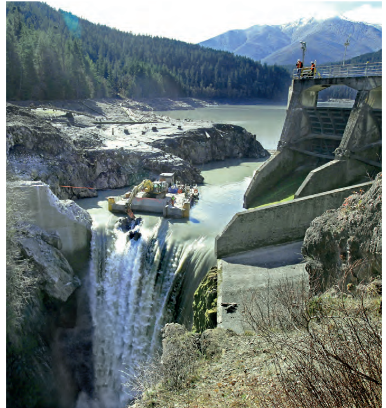
THE 64 M HIGH GLINES CANYON DAM (AKA UPPER ELWHA DAM) DURING REMOVAL © US National Park Service
